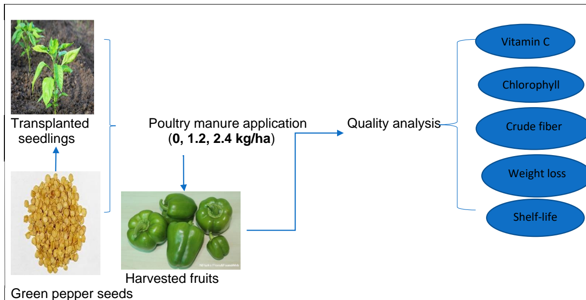
Figure 1. Flow chart of different poultry manure rates on the postharvest quality and shelf-life of green pepper ( Capsicum annuum ) fruits.
