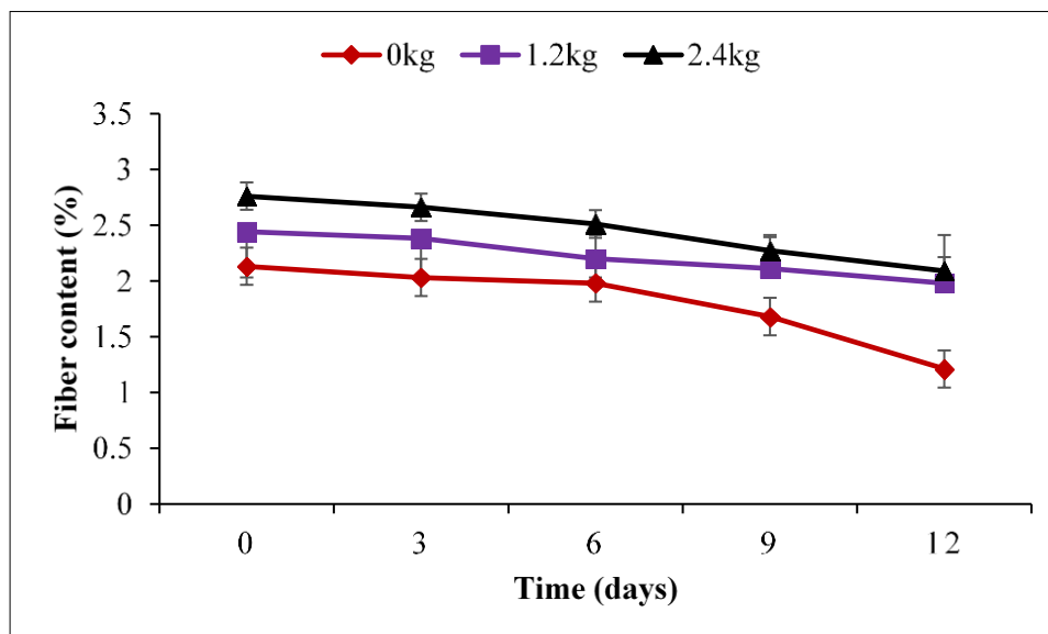
Figure 5. Effect of poultry manure rates on the crude fibre content in green pepper fruits after harvest and during storage.
