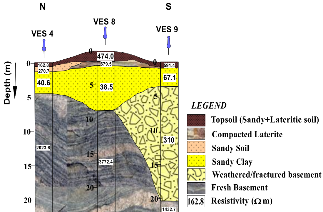
Figure 2c. Geo-electric section of profile C.
